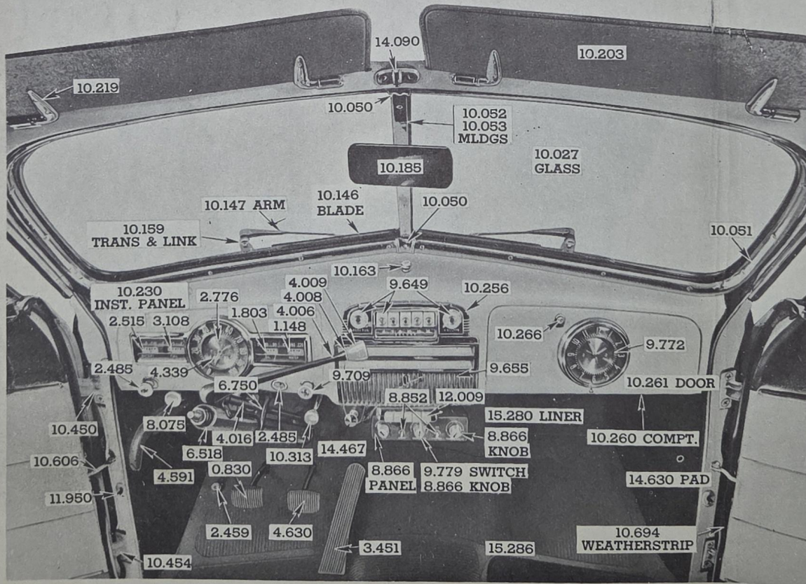
1948 DRIVING COMPARTMENT
