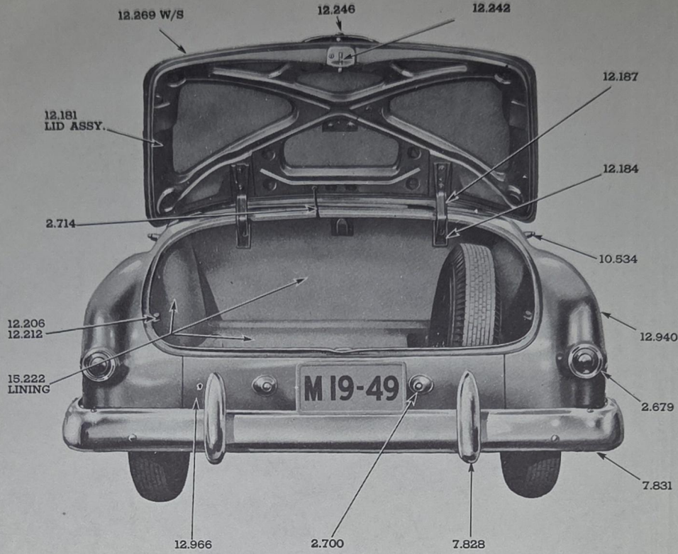
1949 REAR COMPARTMENT
